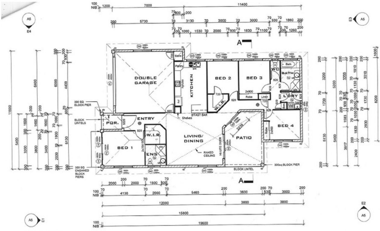
FLOOR PLAN 1:100
